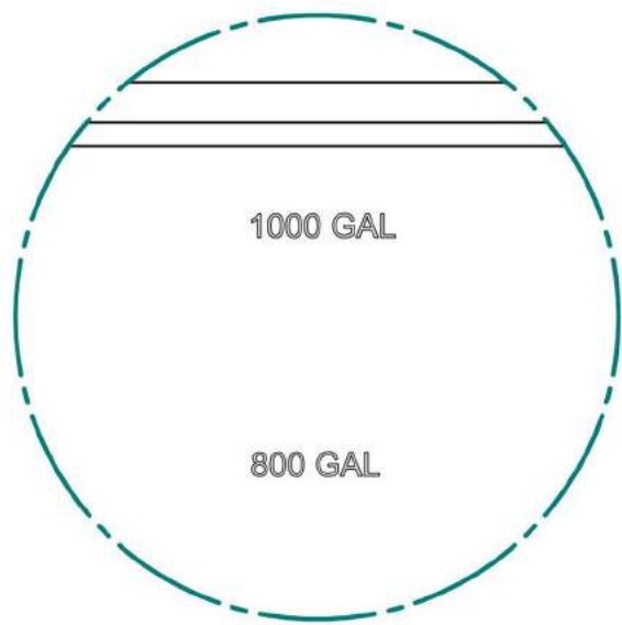
DETAIL B Typical Tank Markings and Graduation
