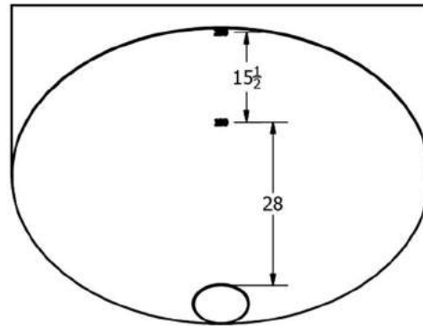
SECTION B-B SCALE 1:20
