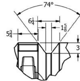
DETAIL B SCALE 1 / 11
