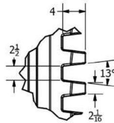
DETAIL C SCALE 1 / 11
