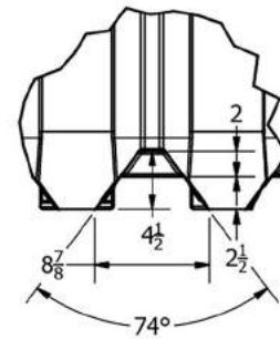
DETAIL A SCALE 1 / 11
