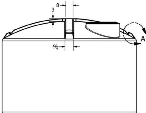
DETAIL A SCALE 0.06 : 1
